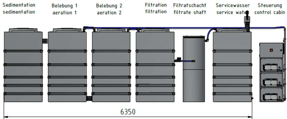
Figure 1: Greywater-Recycling-Plant GWI 7.2 – 7.000
