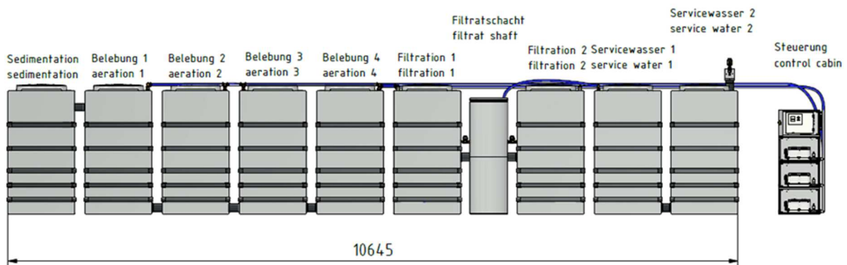
Figure 1: Greywater-Recycling-Plant GWI 20.2 – 20.000
