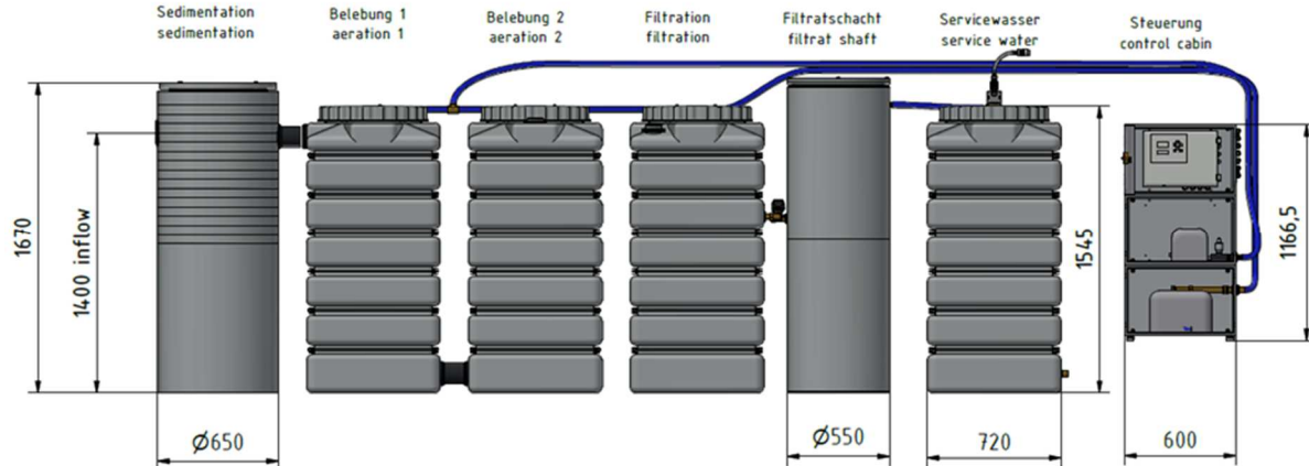
Figure 1: Greywater-Recycling-Plant GWI 2.3 – 2.000
