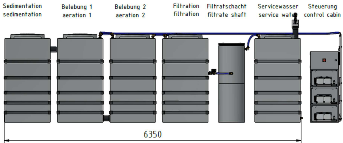
Figure 1: Greywater-Recycling-Plant GWI 10.2 – 10.000
