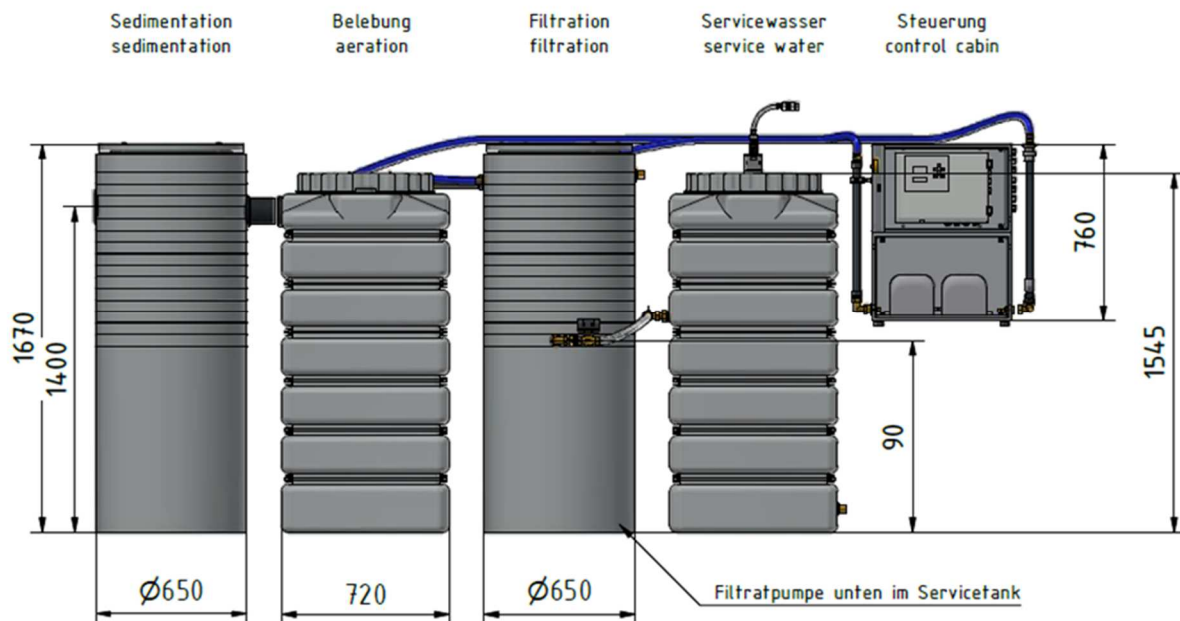
Figure 1: Greywater-Recycling-Plant GWI 1.3 – 1.000
